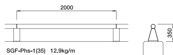
SGF-Phs-1(35)
